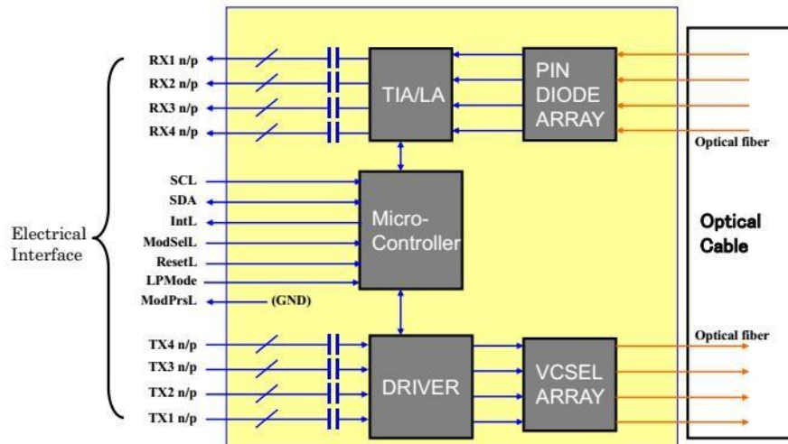
Functional Block Diagram of the QSFP Module
