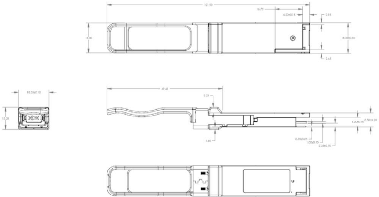
QSFP28-100G-SR4
