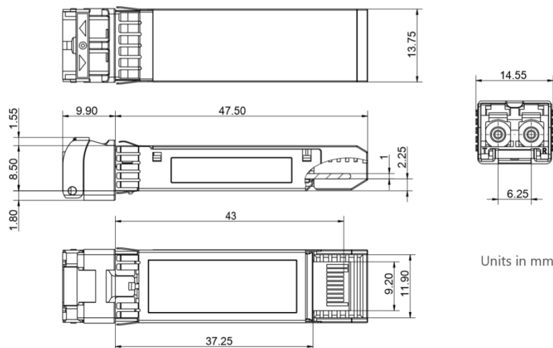
Figure2. Mechanical Outline
