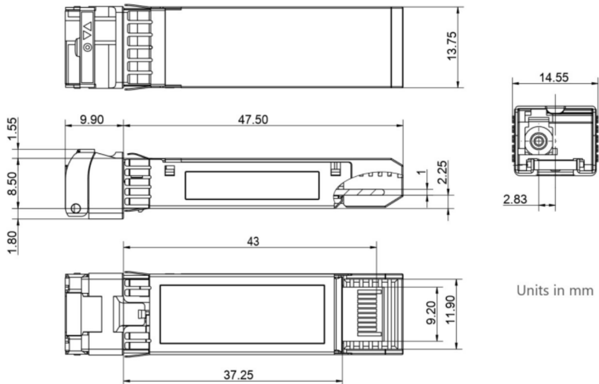
Figure2. Mechanical Outline
