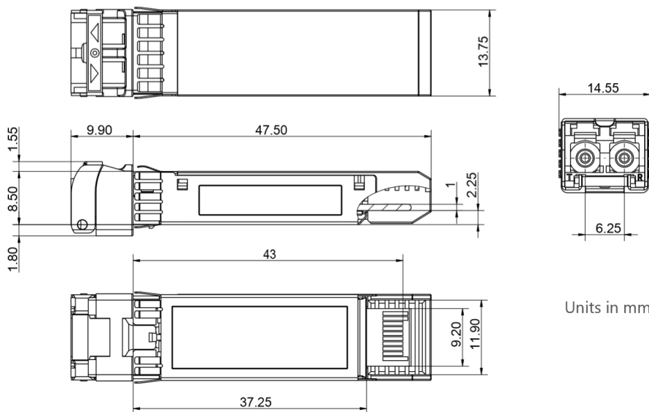
Figure2. Mechanical Outline
