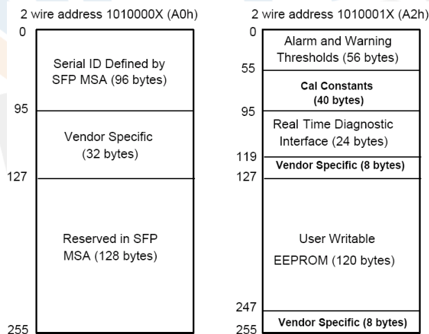
Figure 5 EEPROM Memory Map Specific Data Field Descriptions
