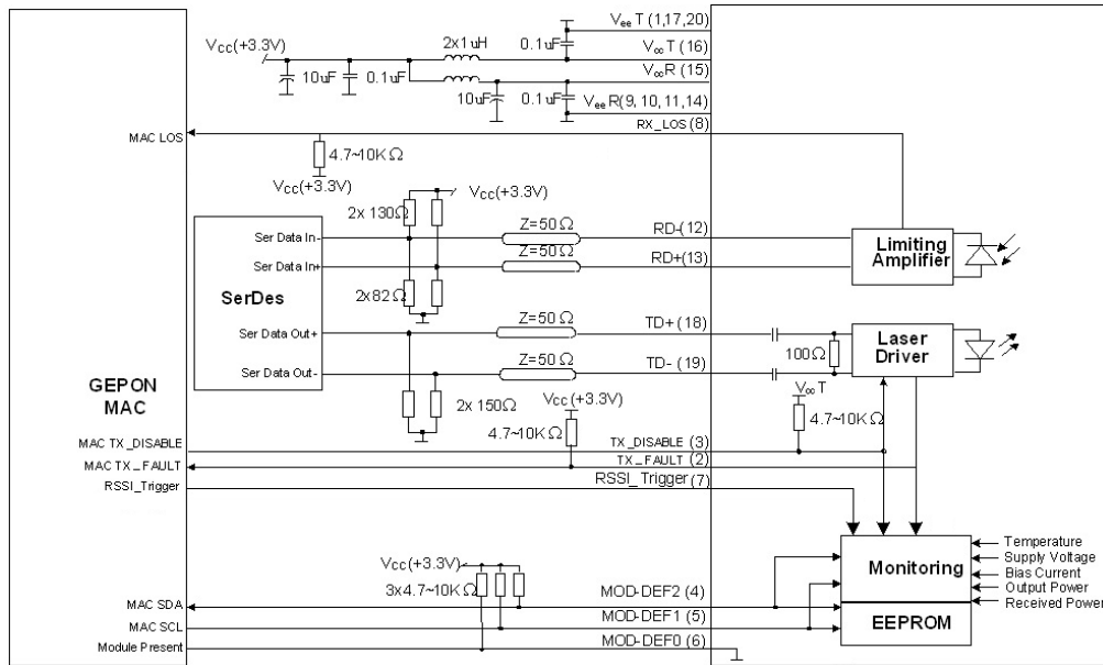
Figure 2 Typical Interface Circuit
