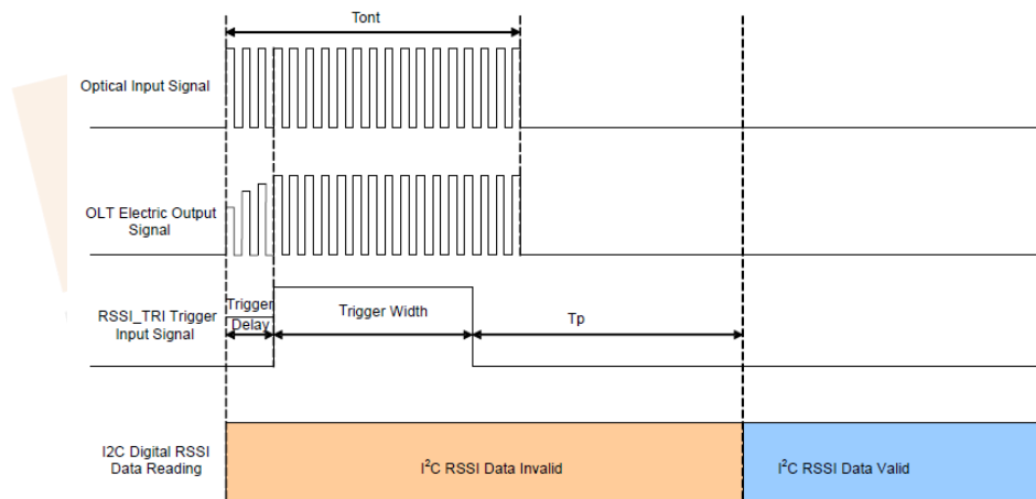
Figure 1 RSSI TIMING SEQUENCE
