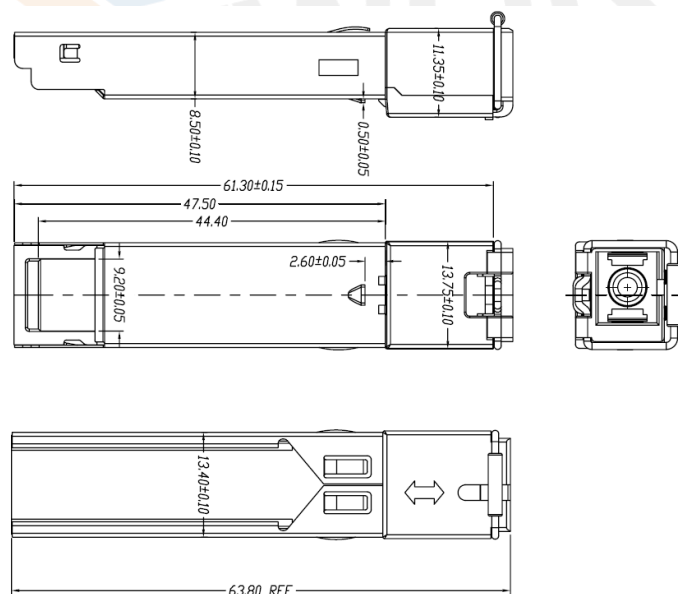
Figure 6 Package Outline
